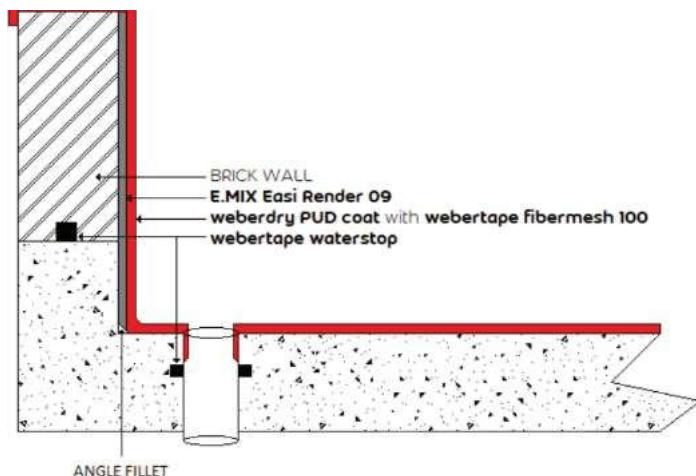
TYPICAL RC FLAT ROOF/CAR PORCH ROOF - EXPOSED SYSTEM
